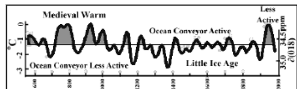
Figure 2 is a plot of paleoclimatic information in the form varying isotopic composition of the ice from cores of Greenland's glaciers. The per mil deviation of the concentration of the heavy isotope 18O in ice compared to standard Mean Ocean Water. Annual ice layers were laid down at a rate of about 30 cm per year throughout this GISP ice core that was 430 m long. Broecker's (1991) Ocean Conveyor periods are noted, too.
