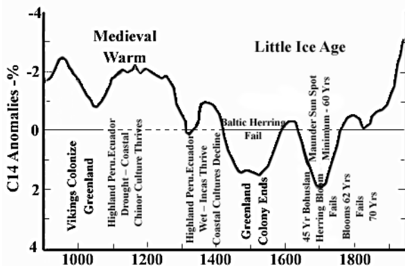
Figure 3 combines the proxy 14C solar activity record of the last 1,100 years. Note that the axis for the solar activity proxy - C14 production - has been reversed. The Maunder minimum refers to the period 1645 – 1715 when very few sunspots were observed on the sun. In this period the production of C14 was very high in agreement with a low solar activity. The periods of approximate rise and fall of colonies of people in both Greenland (Svenmark et al., 1987), and Northern Peru
