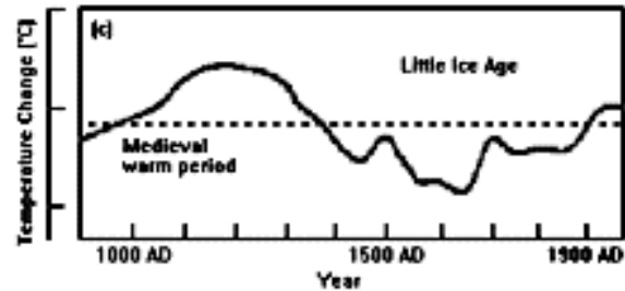
Figure 1c The third image is the record of the last 1,100 years, since beginning of the Medieval Warm Period, when most local societies were self-sustaining. The most recent perturbation from this warming trend is the period that has been called the Little Ice Age. Its effects lasted from ~1450 to ~1850 +/-100 years), depending upon where on Earth people were, and the weather they were accustomed to.
