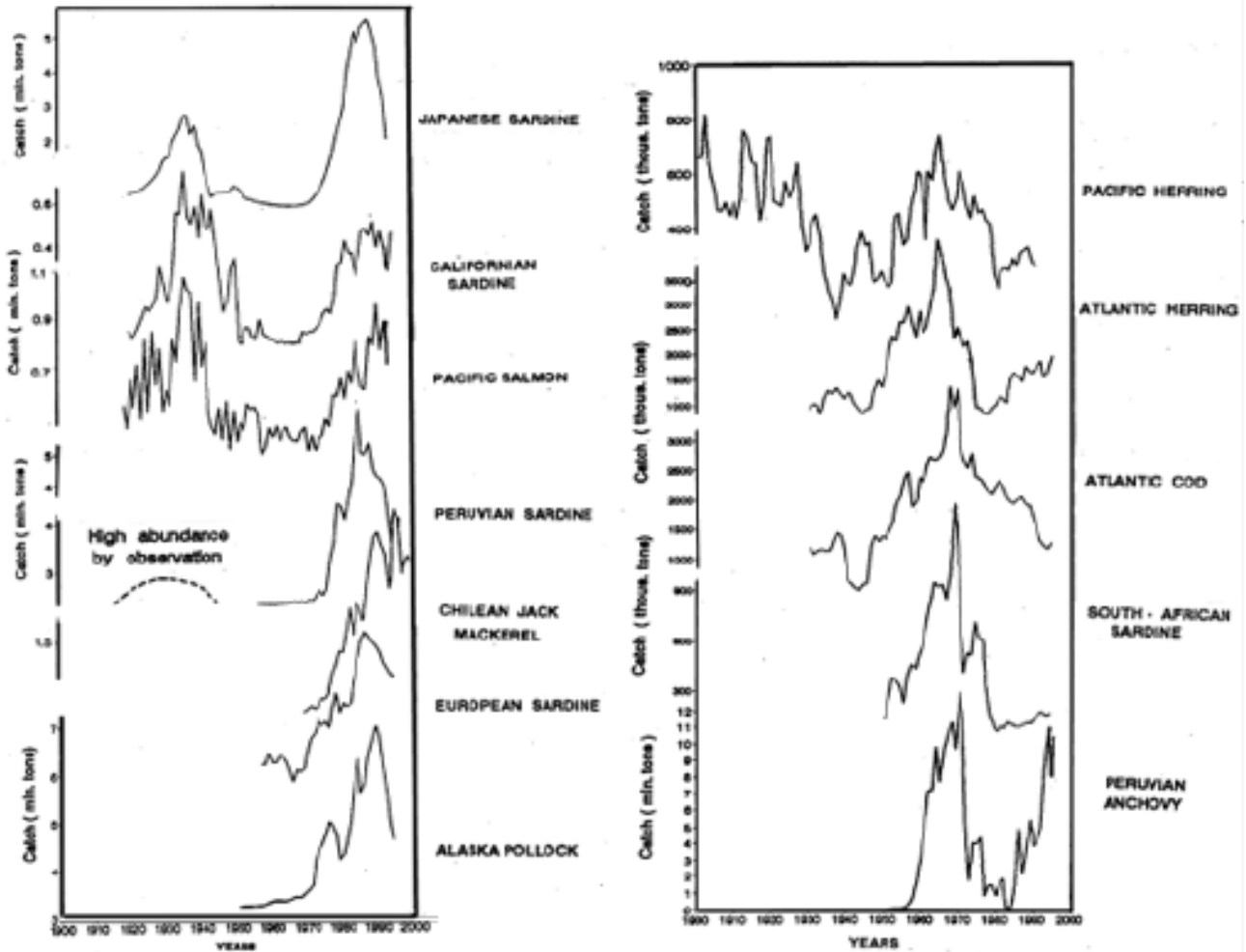
Figure 8 Catch records of the major Warm and Cold epoch fisheries of the Atlantic and Pacific oceans (Klyashtorin and Nikolaev, submitted for Publication in the Encyclopedia of Human Ecology, K. Watt, editor.)
