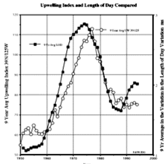
Figure 6 is a plot of Length of Day and the Upwelling Index off San Francisco California. Both were created using nine year running averages, and their ranges scaled to match.
