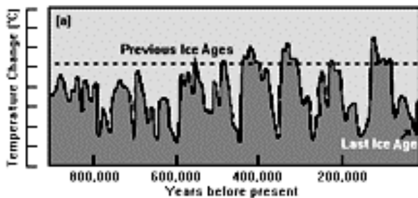
Figure 1a The first is a 900,000 year long picture of the changes in the Earth's surface temperatures, as interpreted by many paleo-scientists, from various proxy records in sedimentary rock strata, laminated ocean bottom sediments, specially selected high and low latitude ice cores, and, more recently, tree rings, and other time-sequenced laminae.
