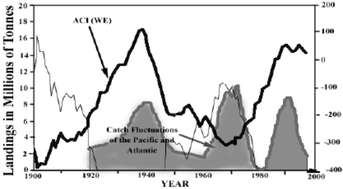
Figure 7 shows the Atmospheric Climate Index of Girs (1971) updated by Klyashtorin and Nikolaev (in review) compared with the catches of the major fisheries of the North Atlantic and Pacific Oceans (c.f., Figure 8, below).
