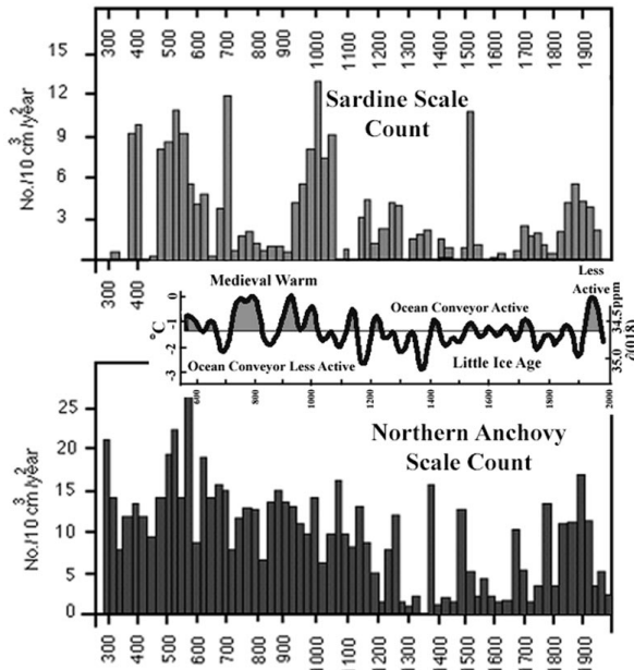
Figure 4 is a plot of the Santa Barbara Basin sardine and anchovy scale counts (as described by Baumgartner et al. (1992) with the 14C record from Figure 3 embedded on the same time scale. Note the coherence of the sardine scale record with warming periods, inferred from the 14C proxy for solar intensity. Needless to say, whatever happened to the Warm Earth after the 11th century has had profound consequences on the production of the California coastal ocean. (c.f., Kawasaki, this volume
