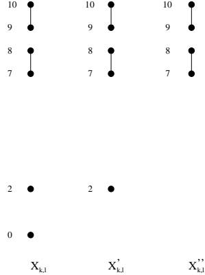
Figure 10. H^*(Th(\xi_k); \mathbb{Z}_3) and \gcd(3, l) = 1
