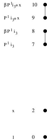
Figure 9. H^*(E_{l^2}; \mathbb{Z}_3) and \gcd(3, l) = 1
