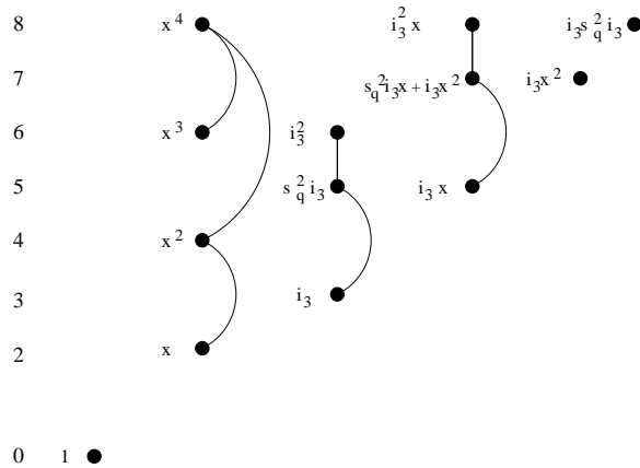
Figure 6. H^*(E_{l^2}) for l even
