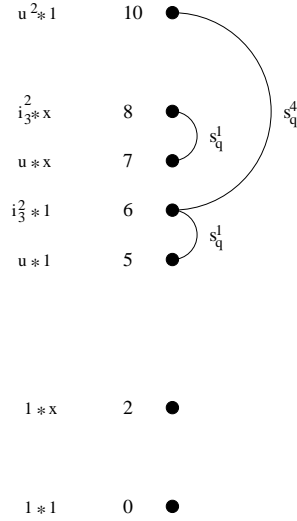
Figure 2. H^*(E_{l^2}) for l odd
