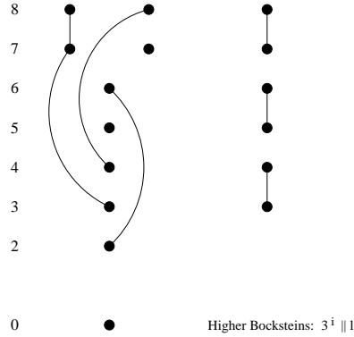
Figure 11. H^*(E_{l^2}; \mathbb{Z}_3) and 3^i || l
