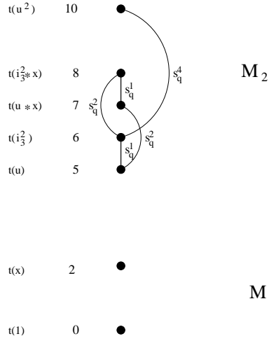
Figure 3. H^*(Th(\xi_k)) for l odd
