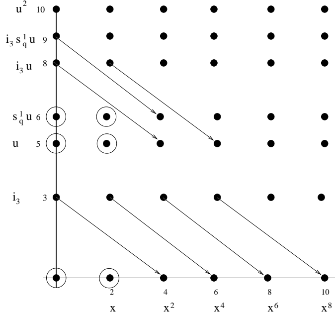
Figure 1. The spectral sequence for E_{l^2}
