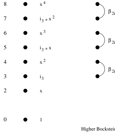
Figure 12. H^*(E_{l^2}; \mathbb{Z}_5) and 5^i || l
