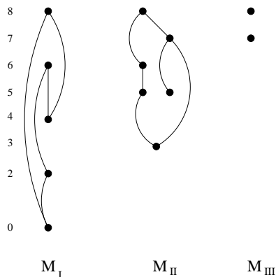
Figure 7. H^*(Th(\xi_k)) for l even
