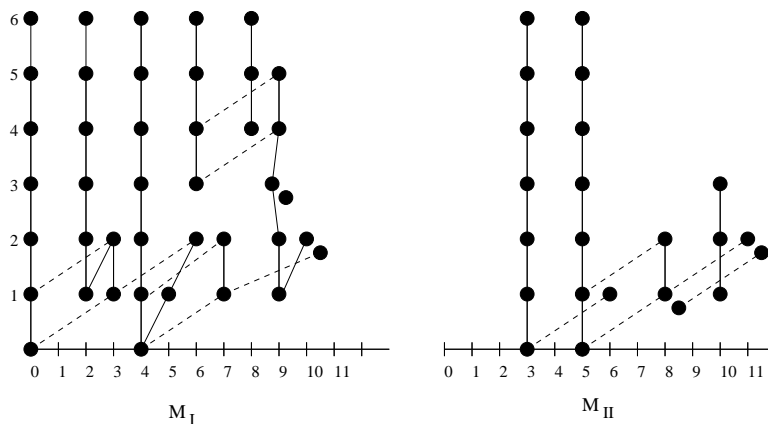
Figure 8. \text{Ext}^{s,t}(M_1; \mathbb{Z}_2) and \text{Ext}^{s,t}(M_2; \mathbb{Z}_2)
