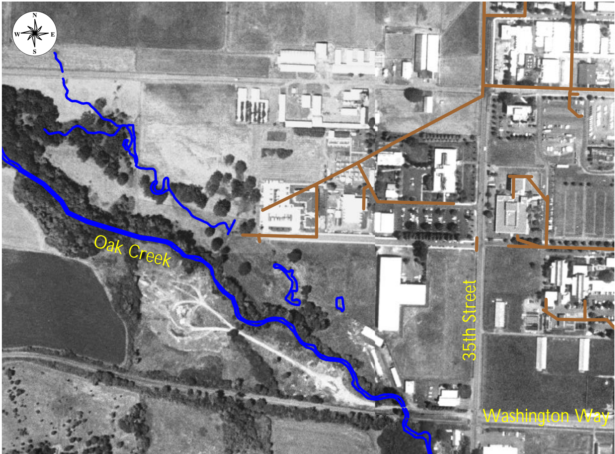
Oak Creek & 35th Street with existing storm lines
