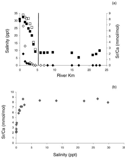
FIGURE 2.—Panel (a) shows the water salinity and Sr:Ca values of samples taken from the entire length of the Salmon River at high and low tide. The dark vertical line represents the position of the highway bridge, which roughly separates the river habitats from the estuarine habitats. The diamonds represent salinity values and the squares Sr:Ca values; open symbols denote values at high tide, closed symbols values at low tide. Panel (b) shows the relationship between water salinity and the Sr:Ca ratio for all Salmon River water samples.
