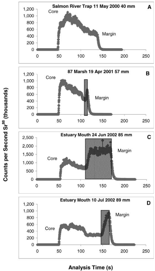
FIGURE 3.—Plots of strontium count rates versus analytical times (otolith radial distances) in four Salmon River Chinook salmon otoliths (A)–(D). The shaded boxes represent periods of estuary residence.
